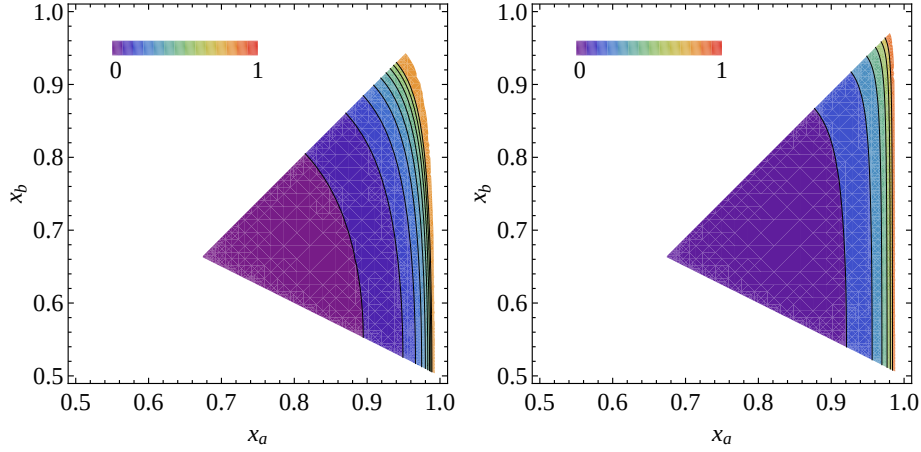
Figure 1: The differential cross sections of e^+e^- \rightarrow q\bar{q}g as a function of x_1 and x_2 , assuming gluon is a vector/scalar particle in left/right diagram.
