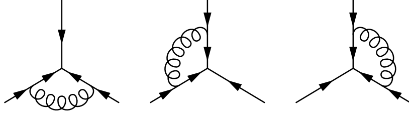
Figure 1: 1-loop QCD correction to the effective operator of proton decay.
