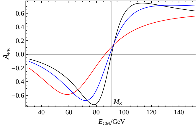
Figure 4: The forward-backward asymmetry A_{FB}^f as a function of center-of-mass energy E_{CM} . The black, blue, and red curves correspond to f\bar{f} = \mu^-\mu^+ , u\bar{u} and d\bar{d} , respectively.
