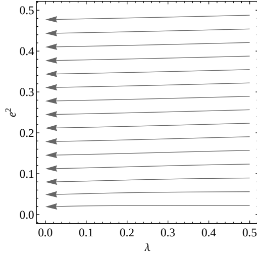
Figure 2: The renormalization group flow of Coleman-Weinberg model.
