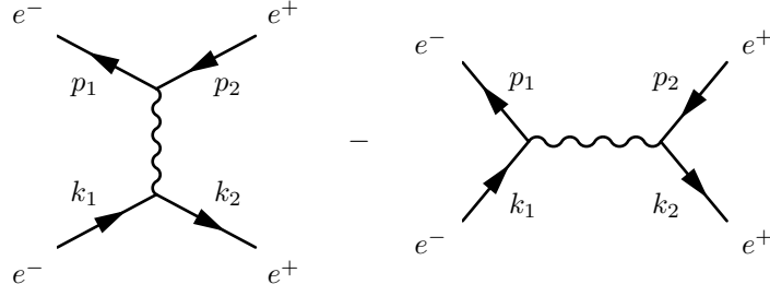
Figure 2: Bhabha scattering at tree level. All initial momenta go inward and all final momenta go outward.
