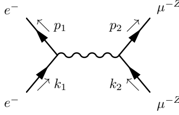
Figure 1: The scattering of an electron by a charged heavy particle \mu^{-Z} . All initial momenta go inward and all final momenta go outward.
