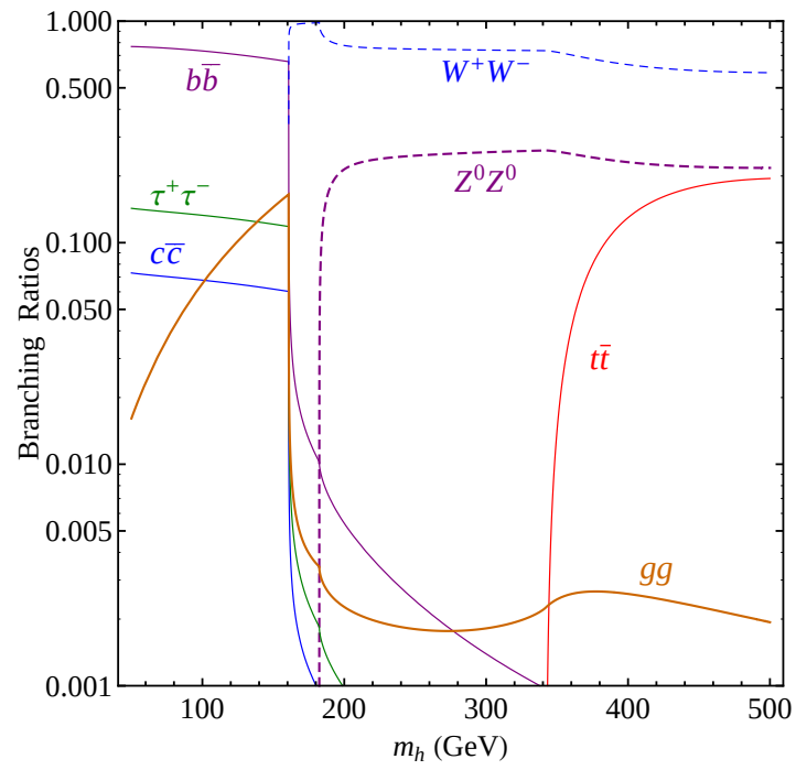
Figure 2: The Higgs decay branching fractions of t\bar{t} , b\bar{b} , c\bar{c} , \tau^+\tau^- , WW , ZZ and gg channels, as functions of Higgs mass.
