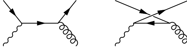
Figure 3: Tree diagrams for the photoproduction of heavy quarks at the parton level.
