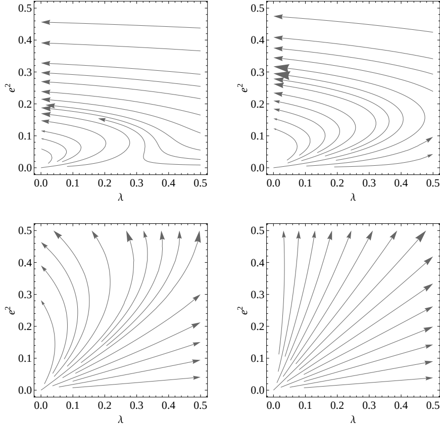
Figure 3: The renormalization group flows of Coleman-Weinberg model in d = 4 - \epsilon spacetime dimensions, with \epsilon = 0.005, 0.01, 0.1 and 1 in the upper-left, upper-right, lower-left and lower-right diagram, respectively.
