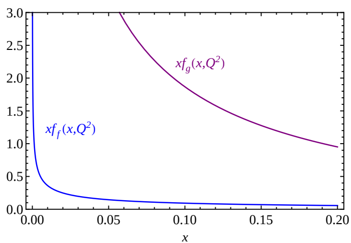
Figure 4: Approximate parton distribution functions at small x with Q = 500\text{GeV} .
