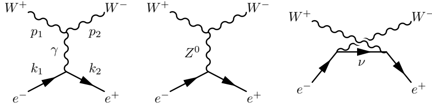
Figure 3: The process e^-e^+ \rightarrow W^+W^- at tree level. All initial momenta go inward and all final momenta go outward.
