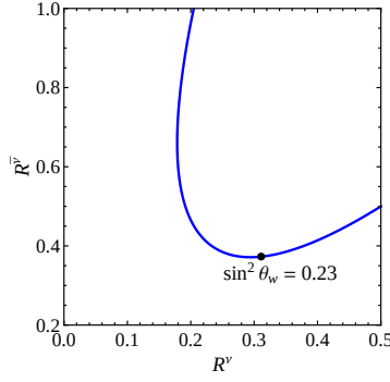
Figure 5: Weinberg's nose with r = 0.4 . See problem 21.4.
