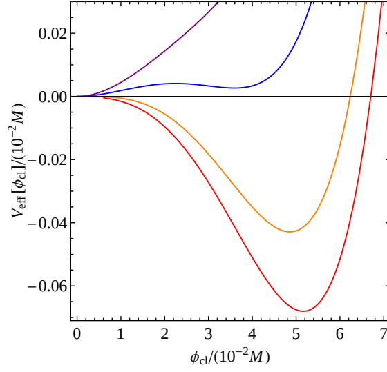
Figure 1: The effective potential V_{\text{eff}} as a function of \phi_{\text{cl}} , with different values of m^2/M^2 = 5 \times 10^{-7} , 2.4 \times 10^{-7} , 0 and -1 \times 10^{-7} from top to bottom, respectively.
