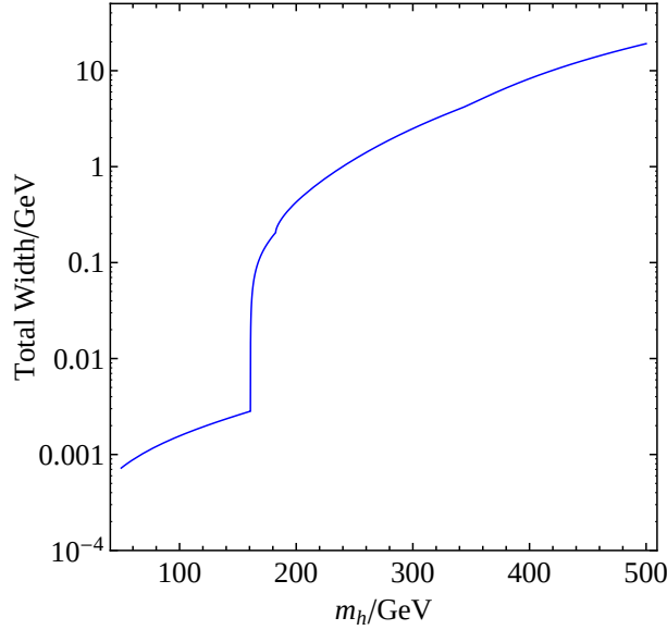
Figure 1: The total width of the Higgs boson as a function of its mass.
