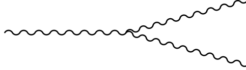
Figure 2: The Gluon splitting process.
