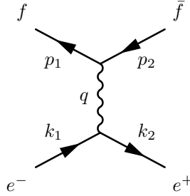
Figure 2: The process of e^+e^- \rightarrow f\bar{f} via the exchange of a photon/ Z^0 in s -channel. The directions of k_i 's and p_i 's are inward and outward, respectively.
