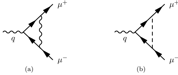
Figure 2: The weak-interaction contributions to muon's EM vertex. These two diagrams contains no neutrino internal lines.
