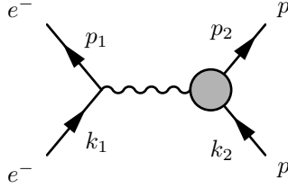
Figure 1: The electron-proton scattering. The blob denotes form factors that includes the effect of strong interaction. All initial momenta go inward and all final momenta go outward.
