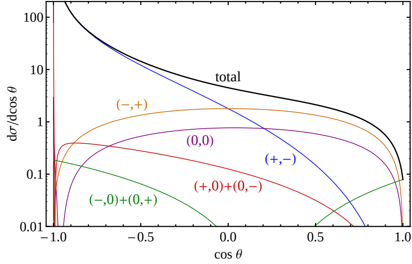
Figure 4: The differential cross section of e^-e^+ \rightarrow W^+W^- with definite helicity as a function of azimuthal angle at s = (1000\text{GeV})^2 .
