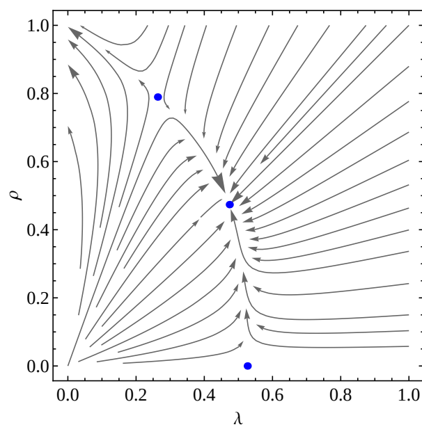
Figure 1: The RG flow of the theory (15) in 4 - \epsilon dimensions with \epsilon = 0.01 . Three nontrivial fixed points are shown by blue dots.
