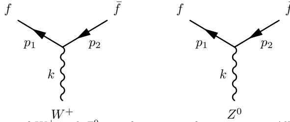
Figure 1: The decay of W^+ and Z^0 into fermion-antifermion pairs. All initial momenta go inward and all final momenta go outward.
