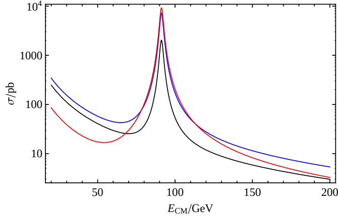
Figure 3: The cross section \sigma(e^+e^- \rightarrow f\bar{f}) as a function of center-of-mass energy E_{\text{CM}} . The black, blue, and red curves correspond to f\bar{f} = \mu^-\mu^+ , u\bar{u} and d\bar{d} , respectively.
