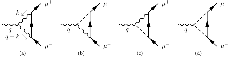
Figure 1: The weak-interaction contributions to muon's EM vertex. These four diagrams contain neutrino internal lines in the loops.
